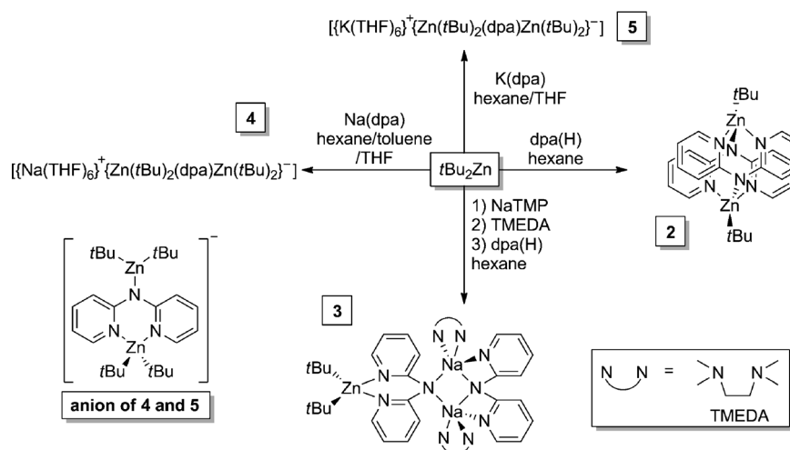
Scheme 1. Synthesis of the neutral zinc dimer 2 , sodium zinczincate 3 , sodium zinczincate 4 , and potassium zinczincate 5 .
